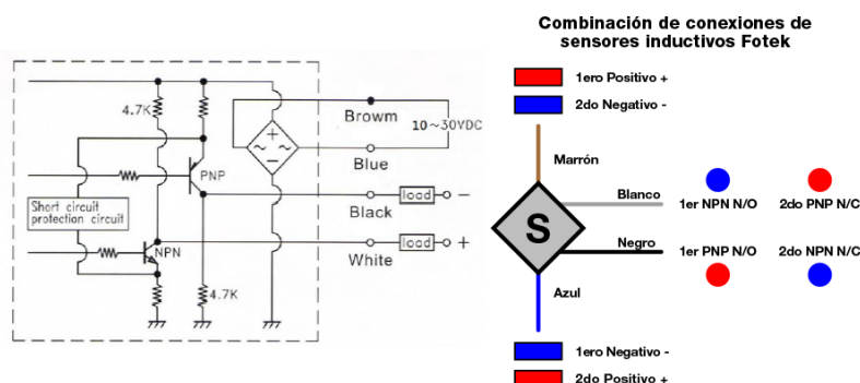
Connection Diagram/接線圖
