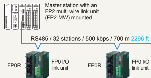
FP0-IOL (AFP0732)
